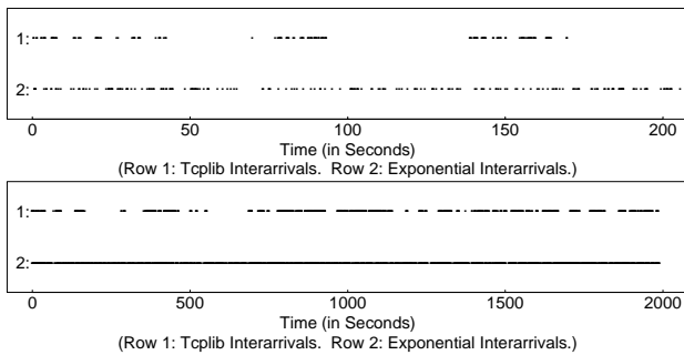
Figure 4: Comparisons between Tcplib and exponential interpacket times.
