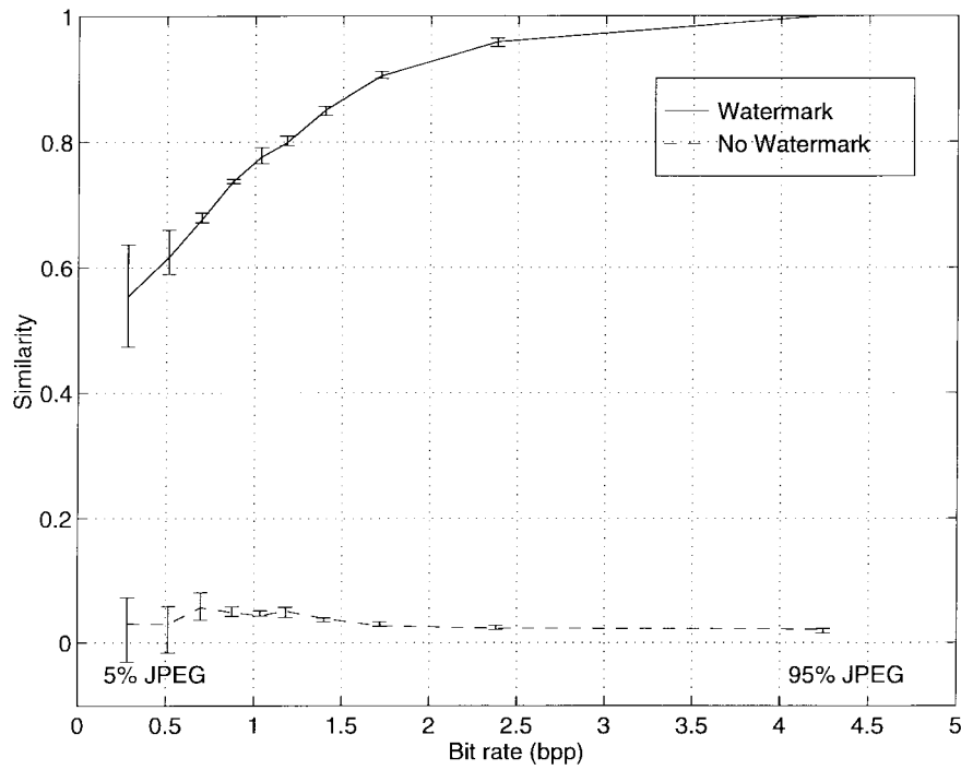
Fig. 9. Detection of watermark in Peppers image after JPEG coding, with qualities from 5 to 95%.
